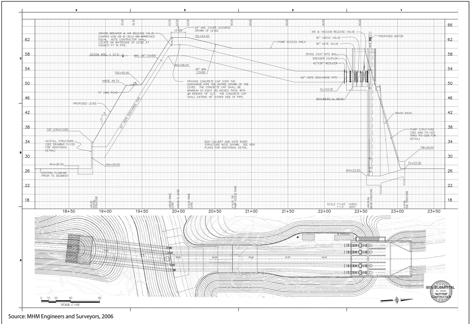
Figure 2 Pump Station #6 Design Plan
